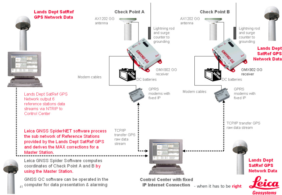
Figure 5: GNSS Network-RTK system architecture
