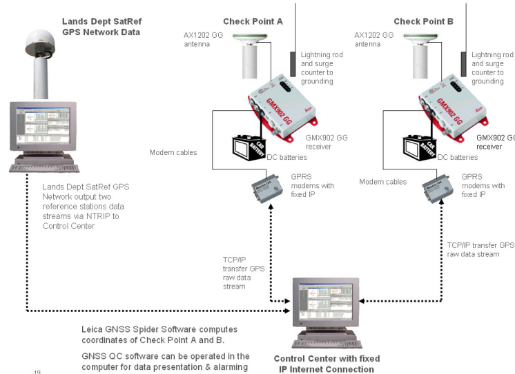
GNSS Single RTK Seawall Monitoring System Diagram
